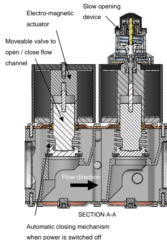
Figure 14 Schematic drawing of VQ400M.
