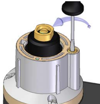
Figure 13 Adjusting opening speed.
