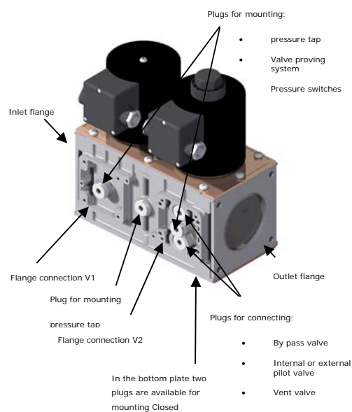
Figure 3 Interfaces for possible accessories
