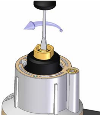
Figure 12 Adjusting step pressure.
